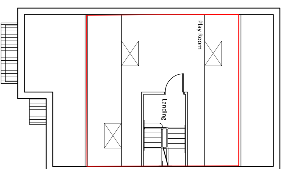
Second Floor
